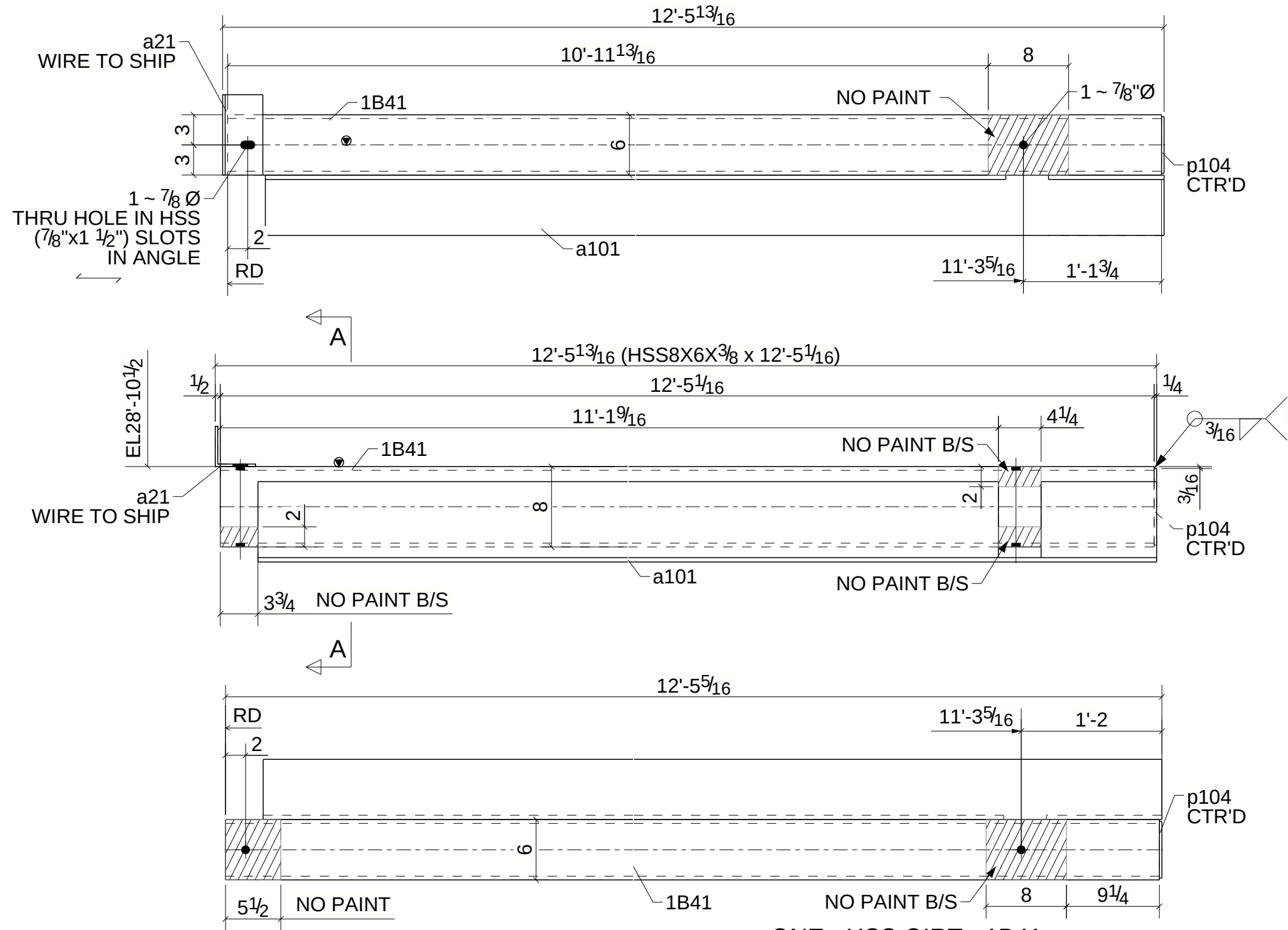
ONE - HSS GIRT - 1B41
